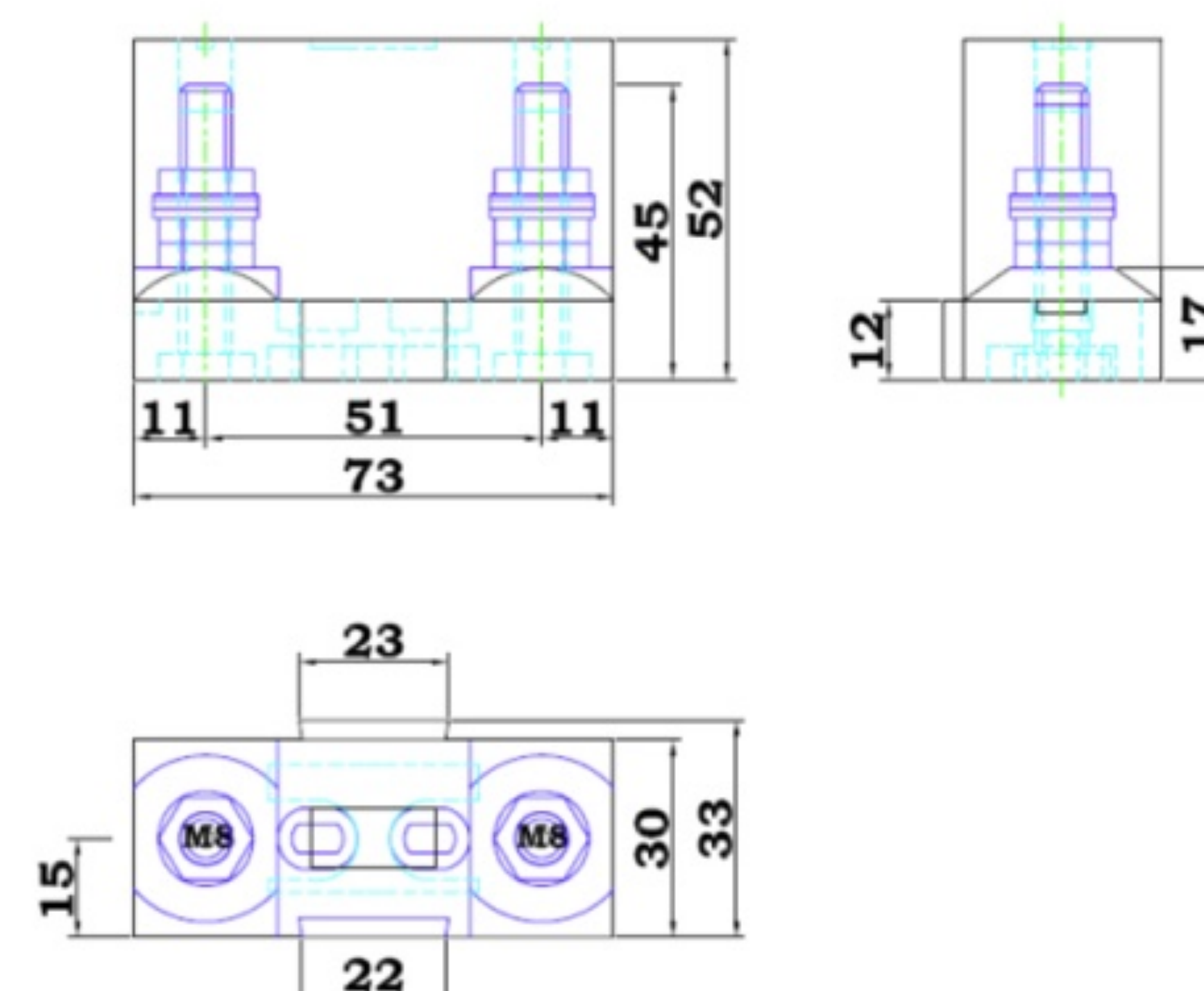
CIP100200100 = Modular fuse holder for Mega-fuse
