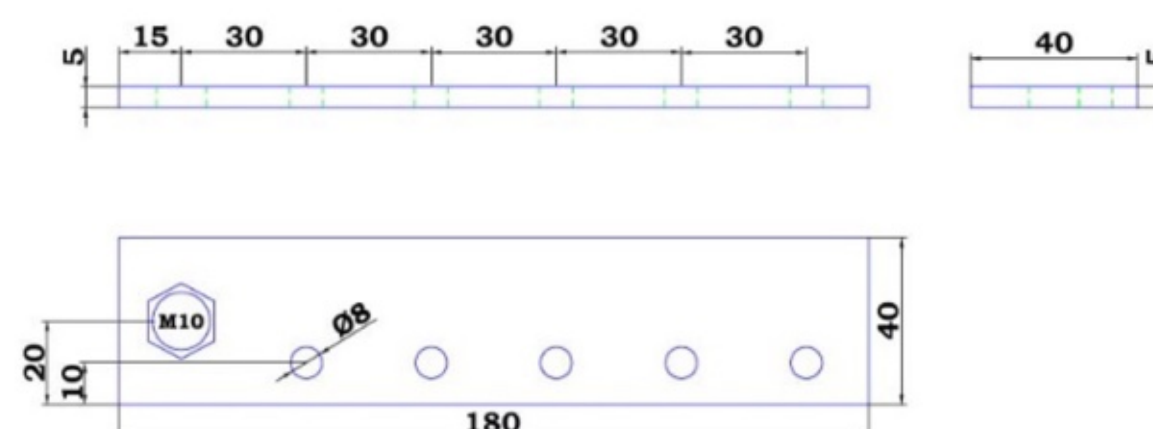
CIP100400060 = Busbar to connect 5 CIP100200100
