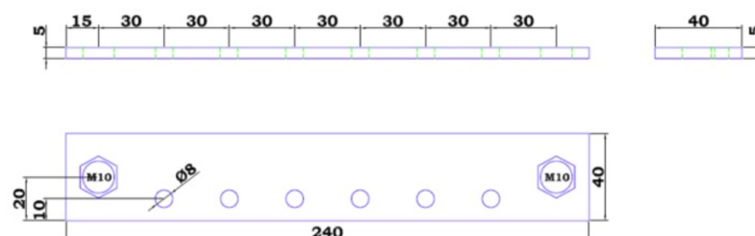
CIP100400070 = Busbar to connect 6 CIP100200100
