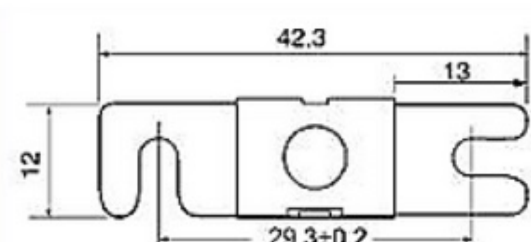
MIDI fuse
