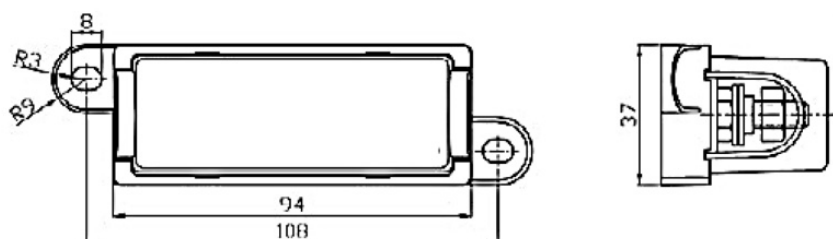
Fuse holder for MEGA fuse
