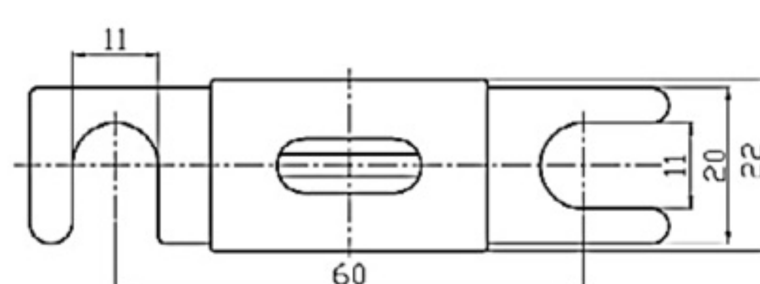
ANL fuse
