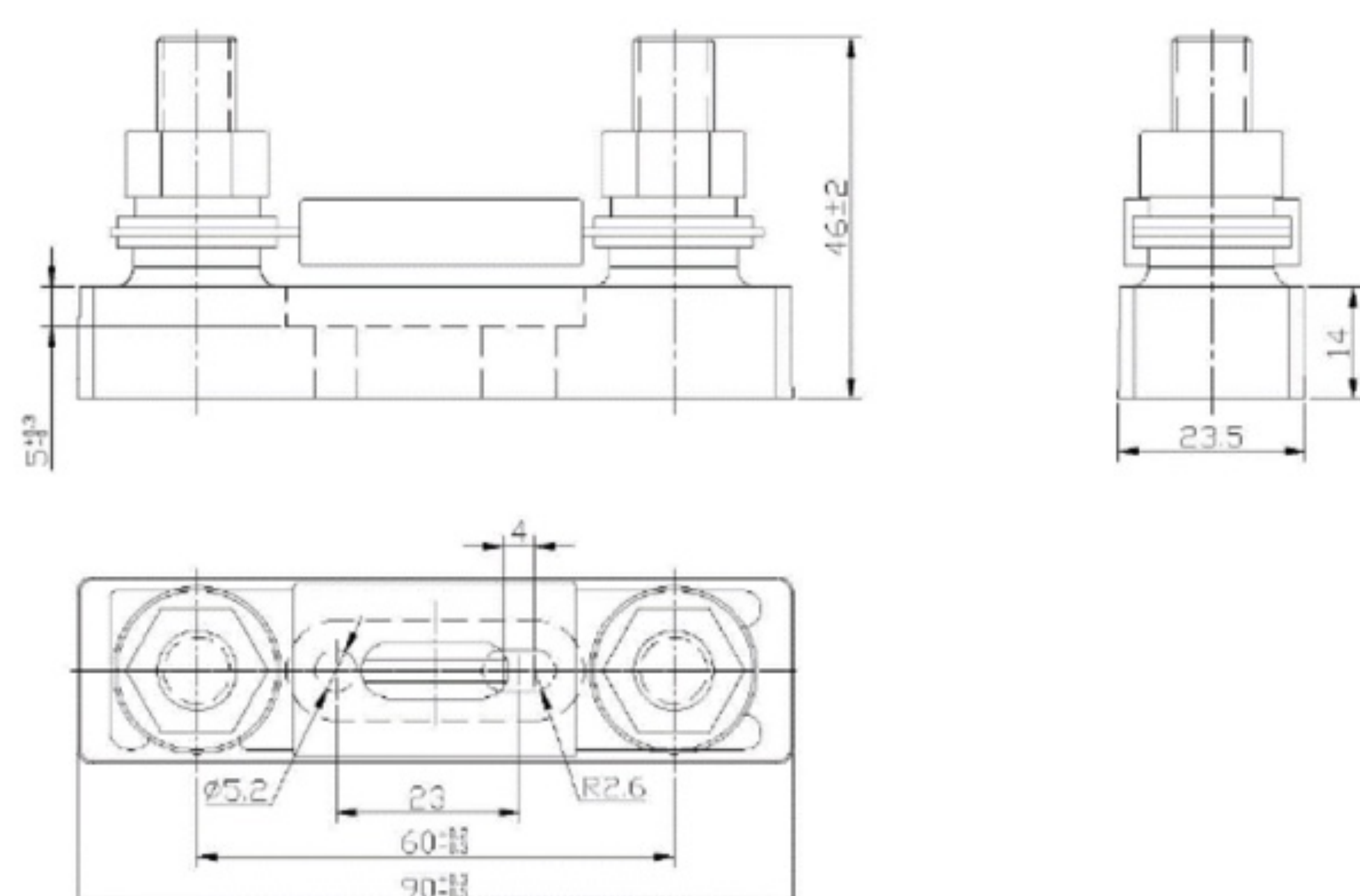
Fuse holder for ANL fuse
