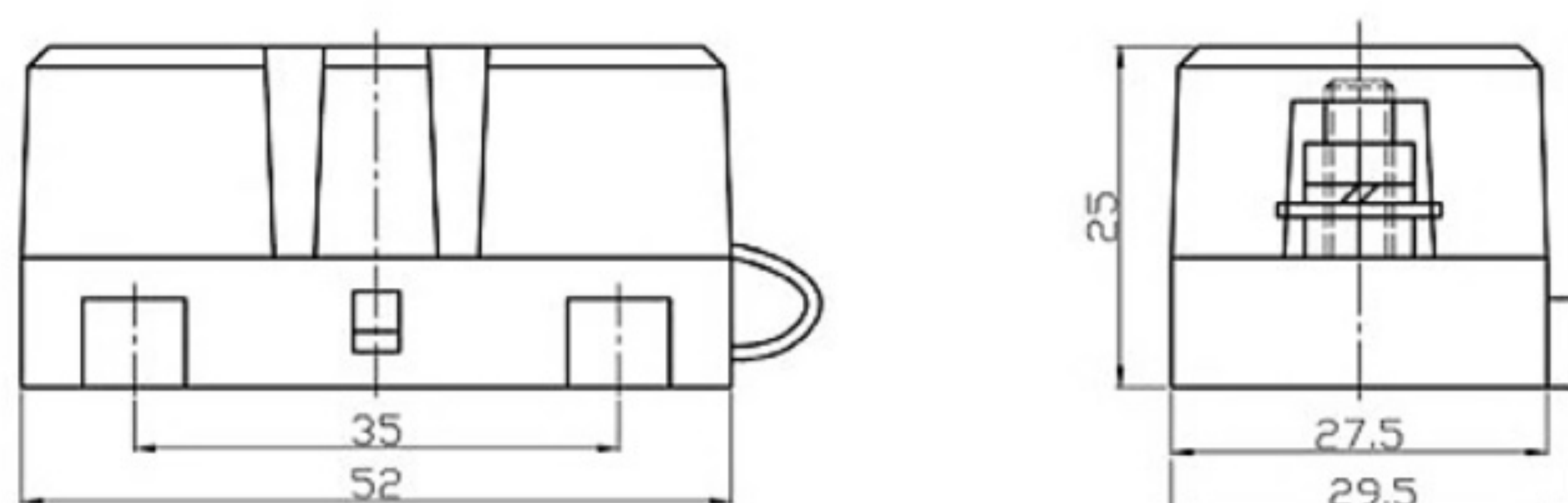
Fuse holder for MIDI fuse
