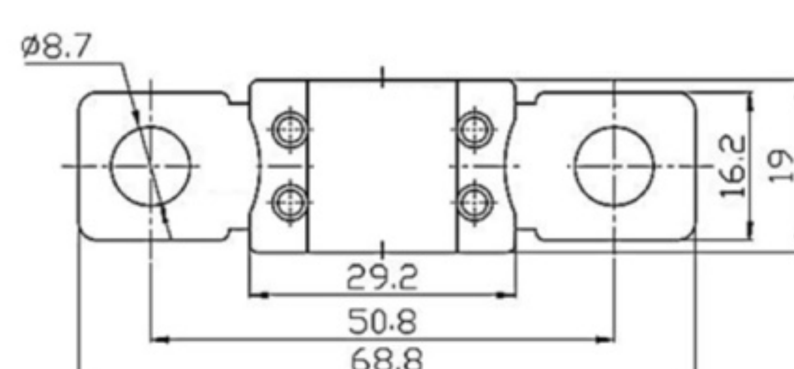
MEGA fuse
