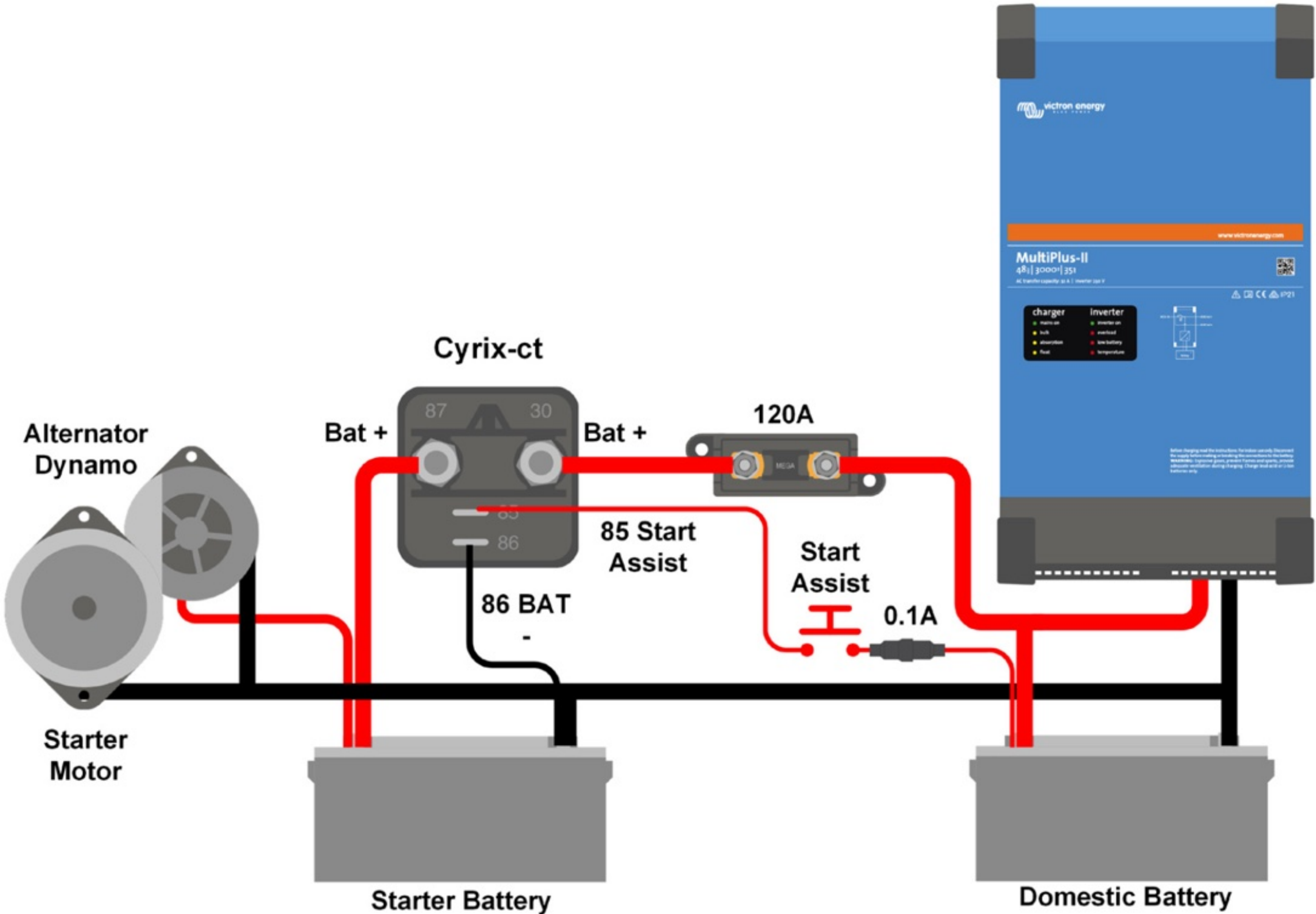
Cyrix-ct 12/24-120: connection diagram
