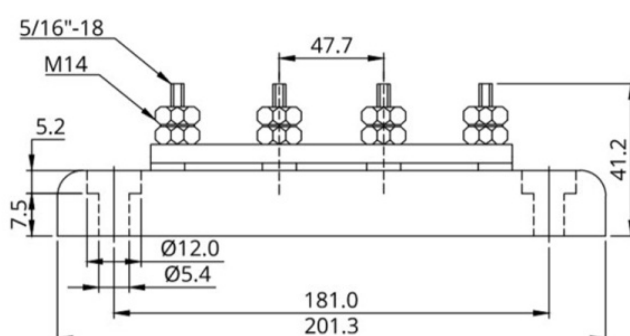
Busbar 250 A with 4 stud terminals and cover
