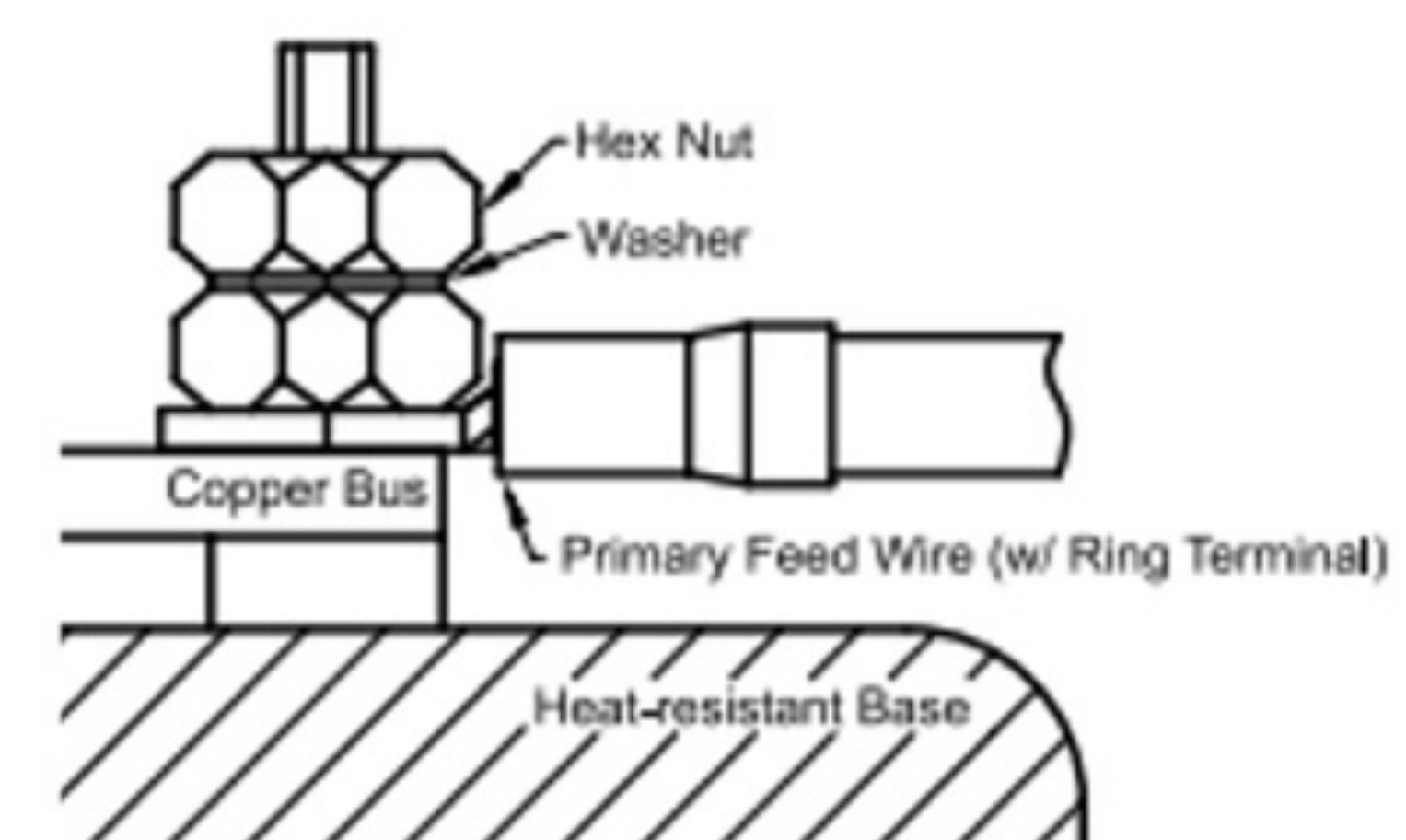
Recommended mounting
