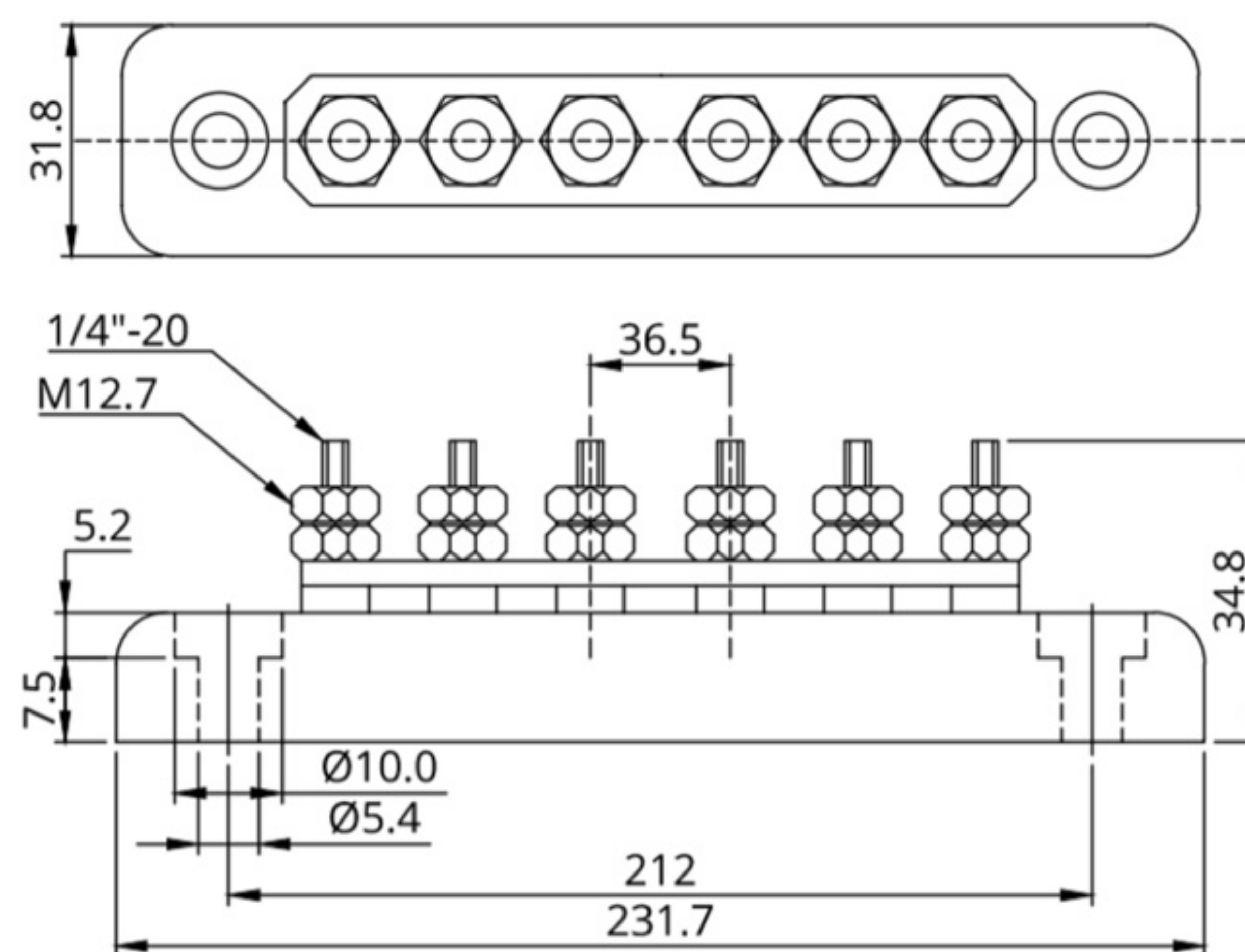
Busbar 150 A with 6 stud terminals (cover not shown)
