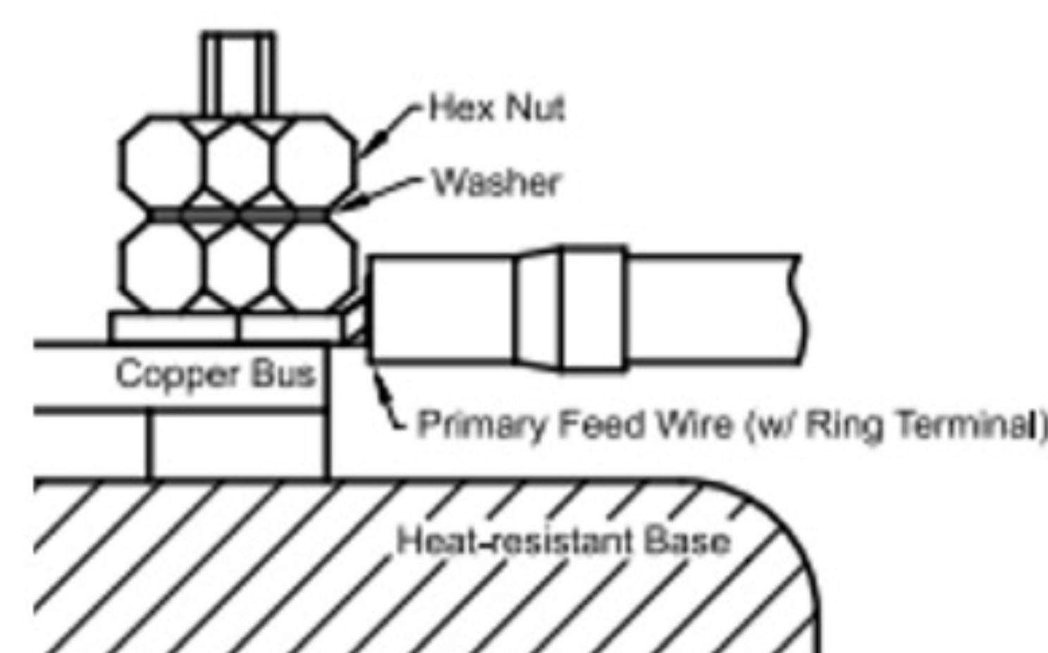
Recommended mounting
