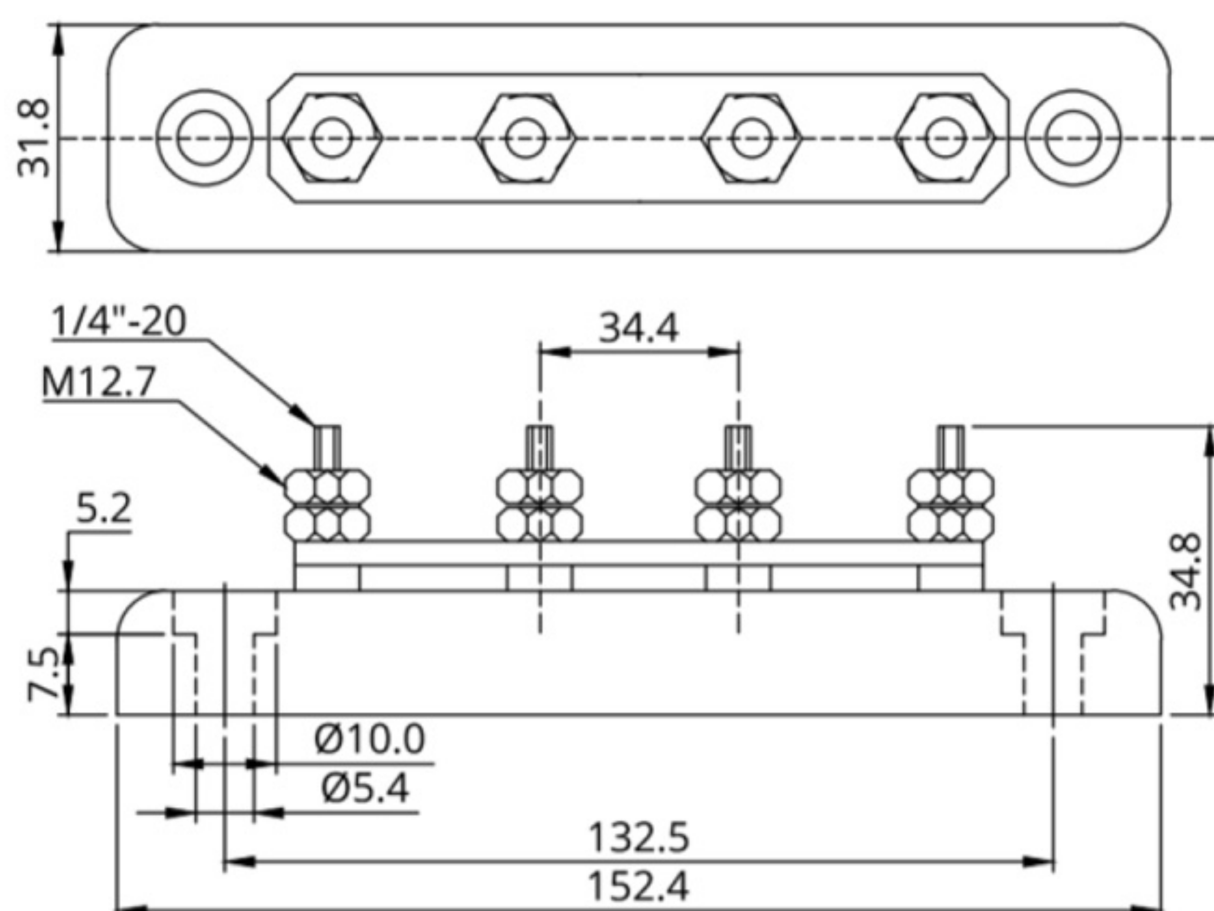
Busbar 150 A with 4 stud terminals and cover
