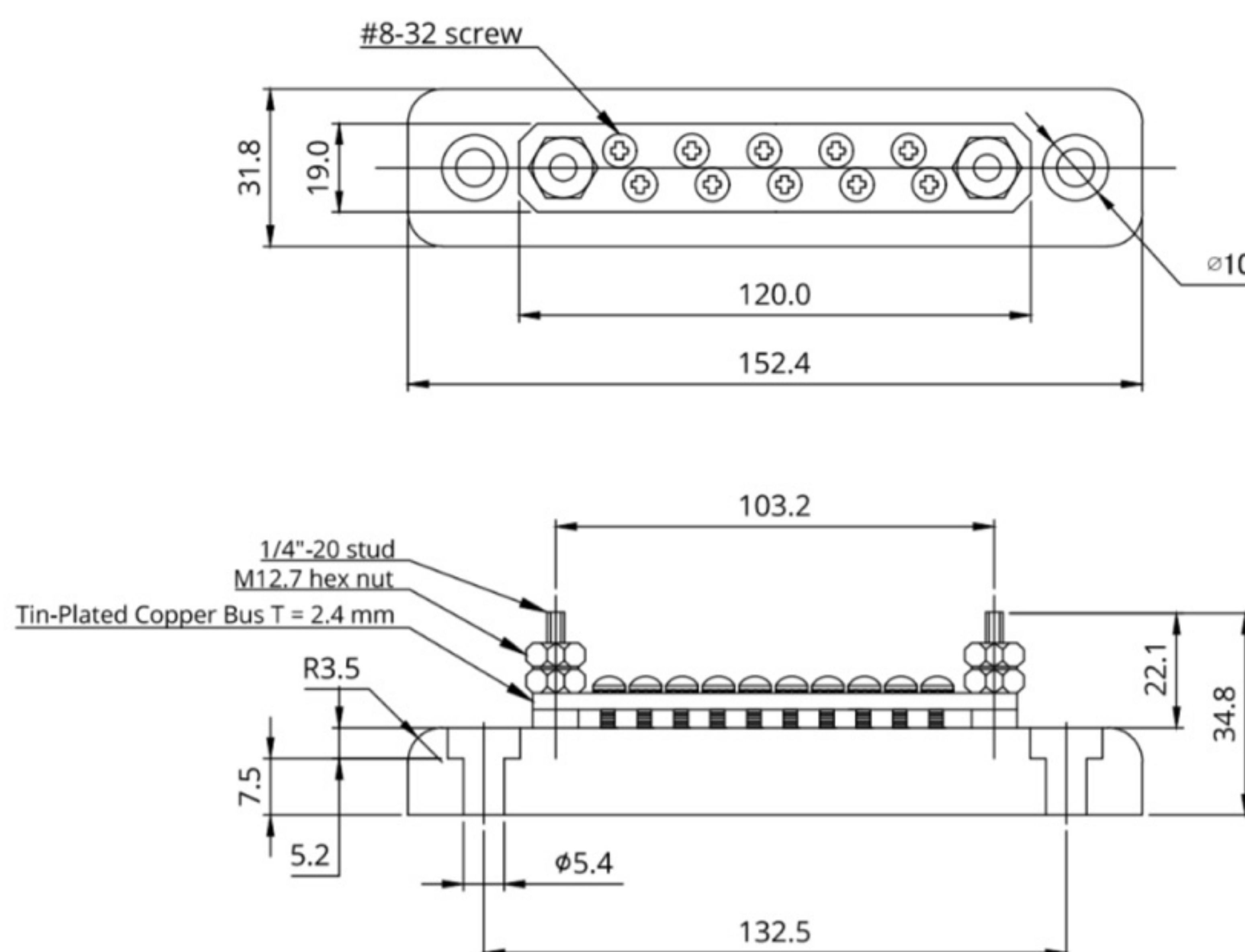
Busbar 150 A 2P with 10 screws
