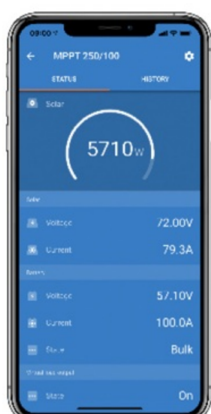
VictronConnect Application
