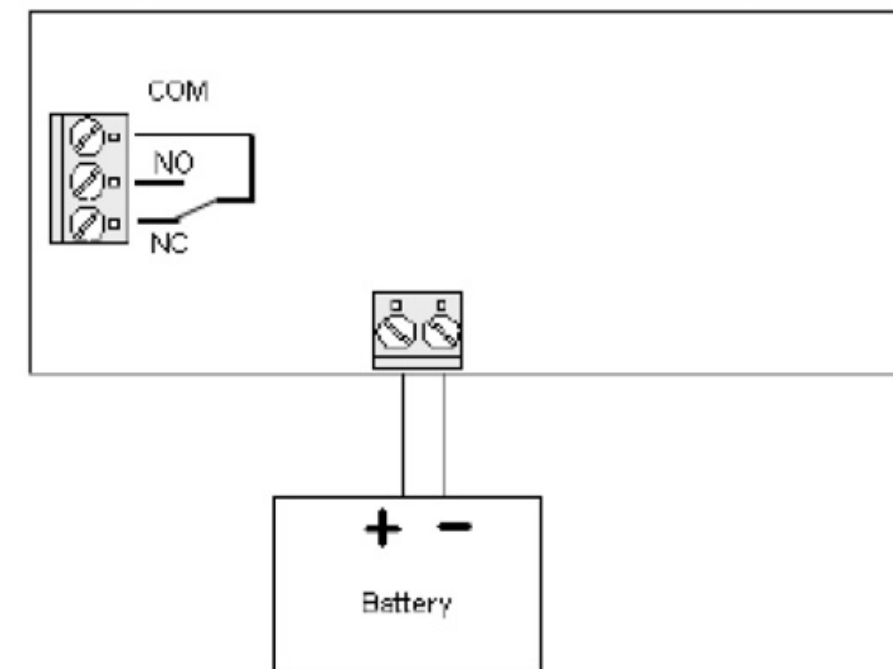
Wiring Diagram
