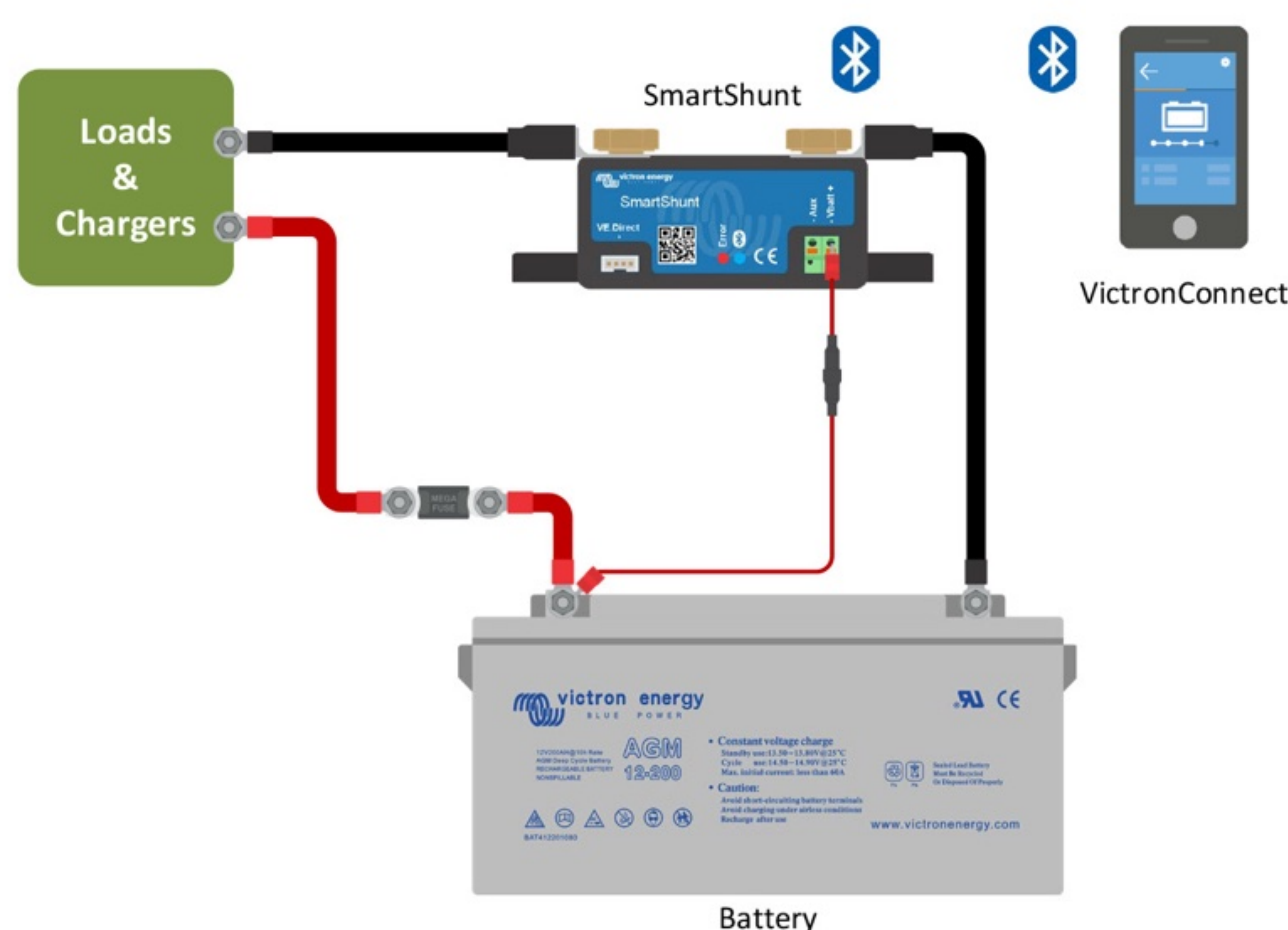
Basic SmartShunt wiring
