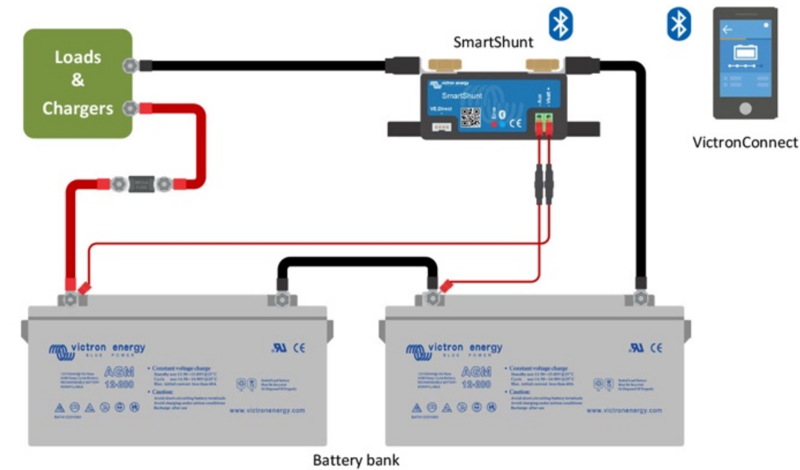
Measuring battery bank midpoint
