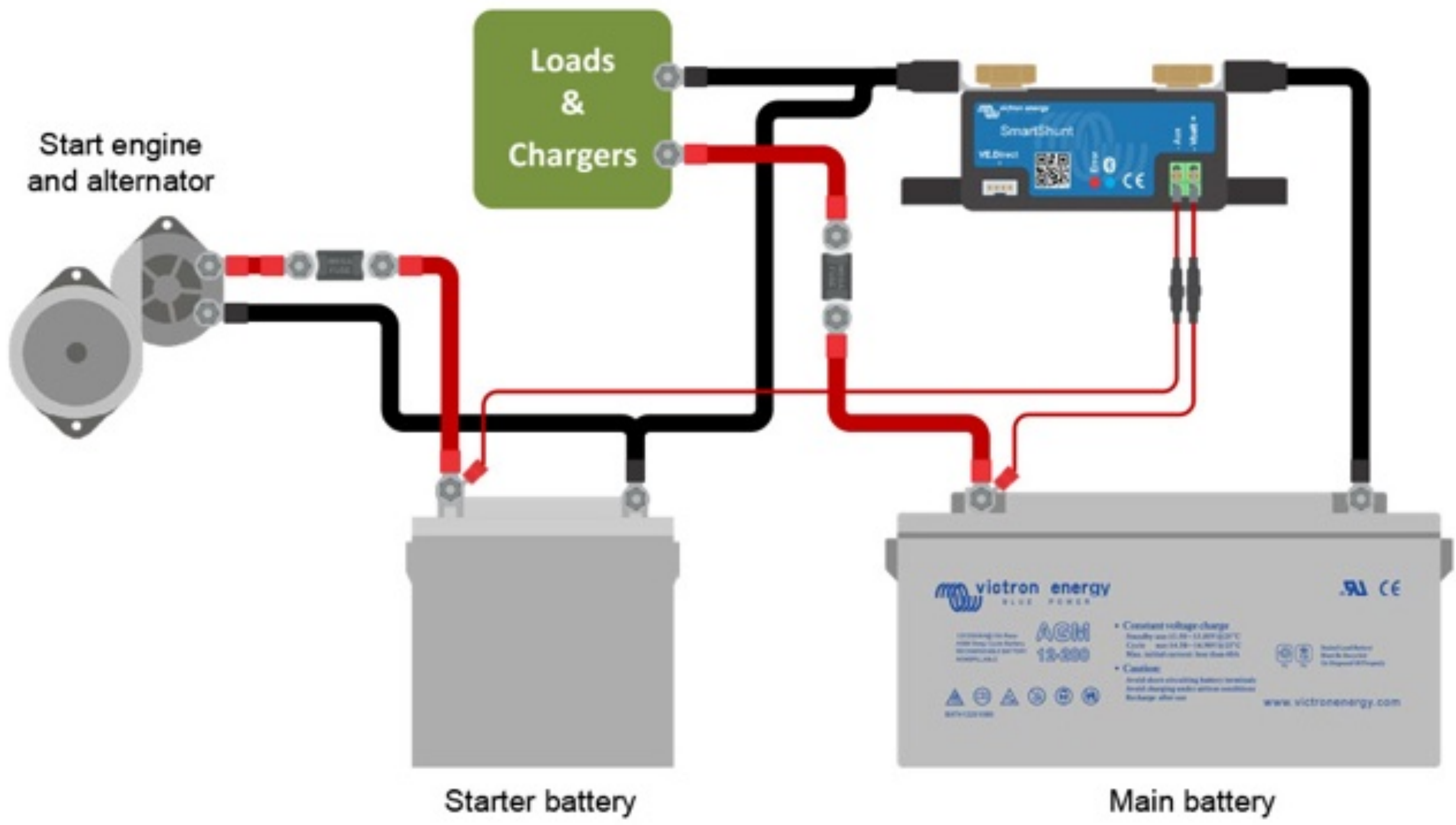
Measuring voltage of the starter battery
