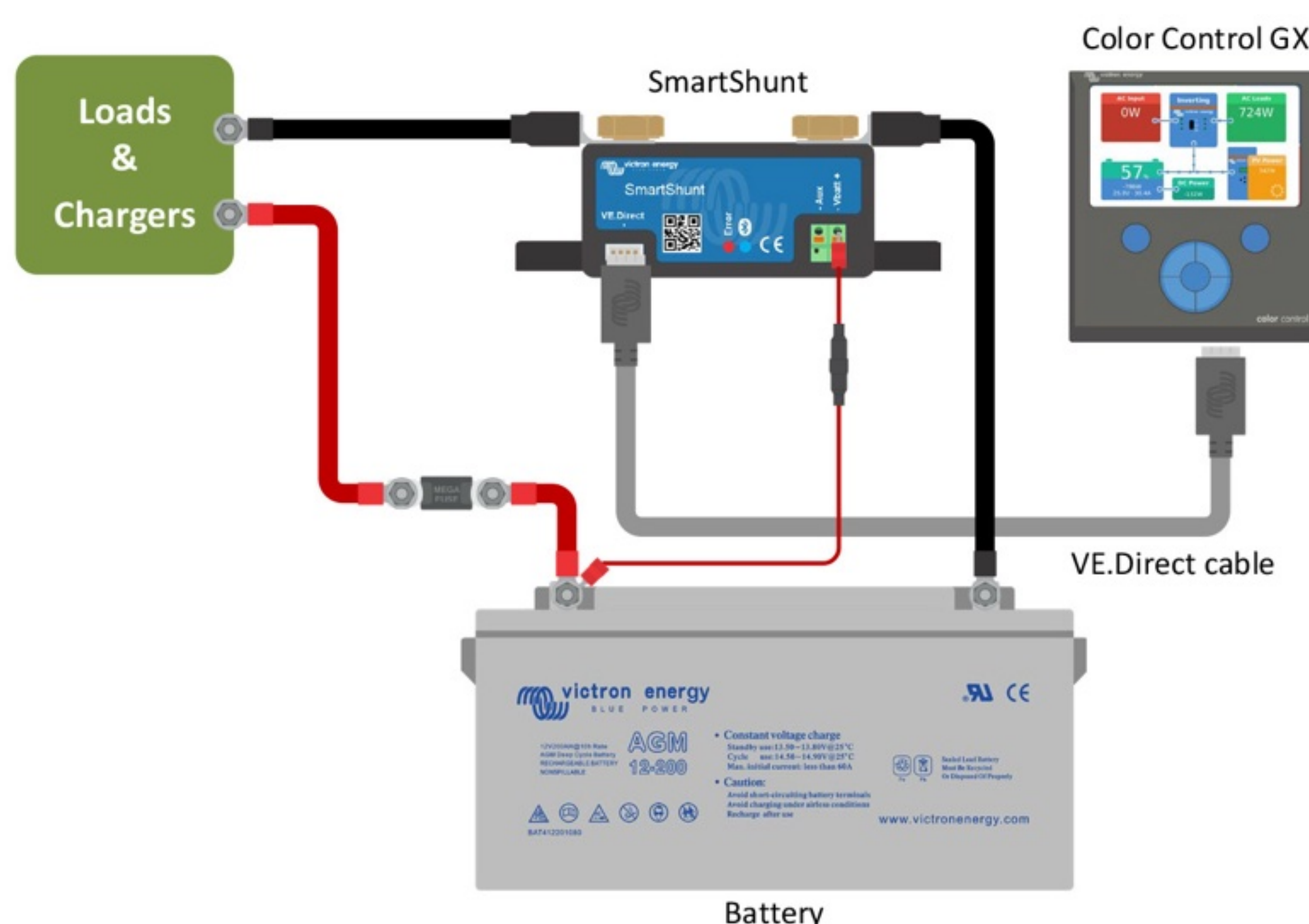
Connecting a SmartShunt to a GX device
