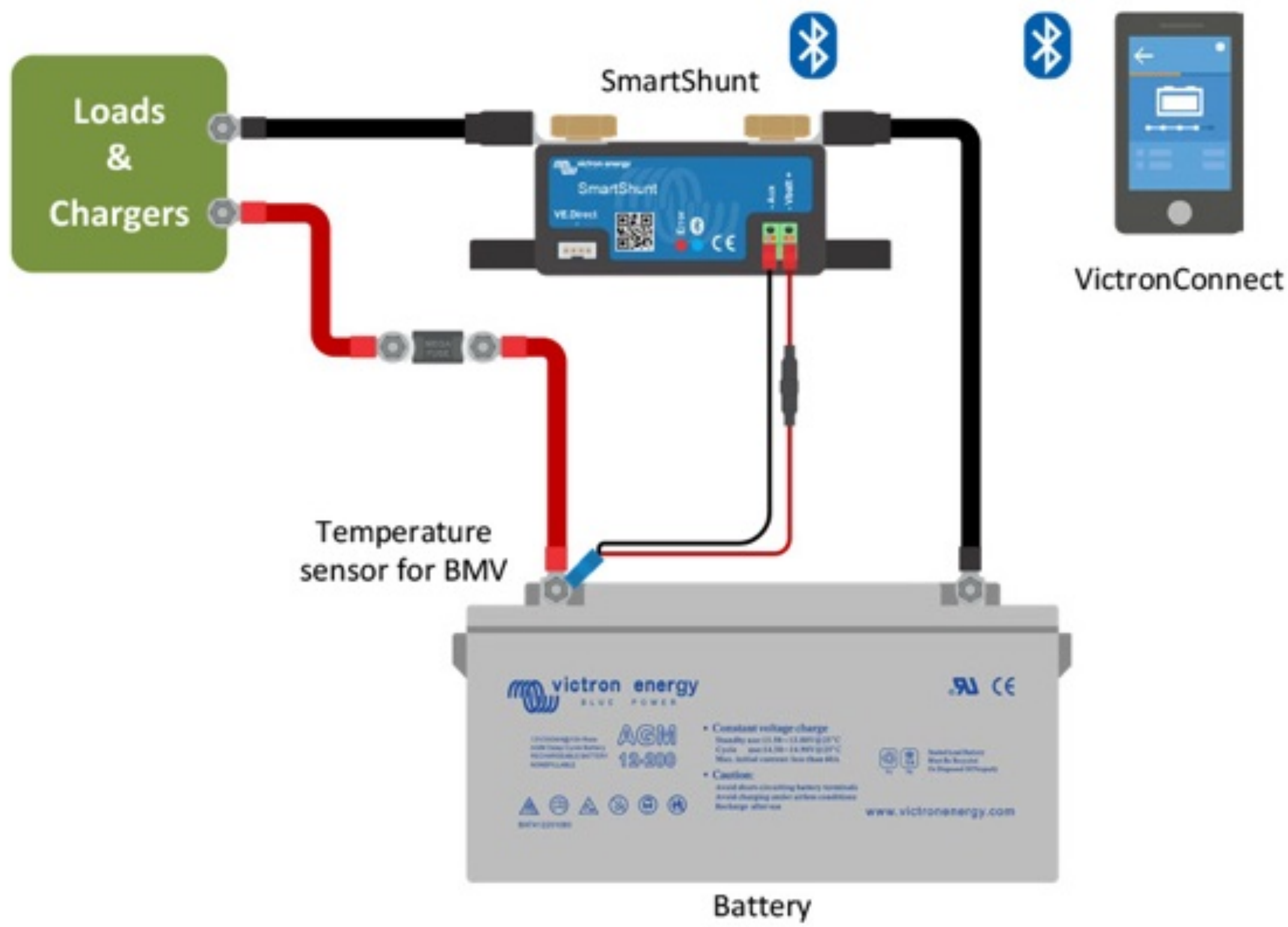
Measuring battery temperature
