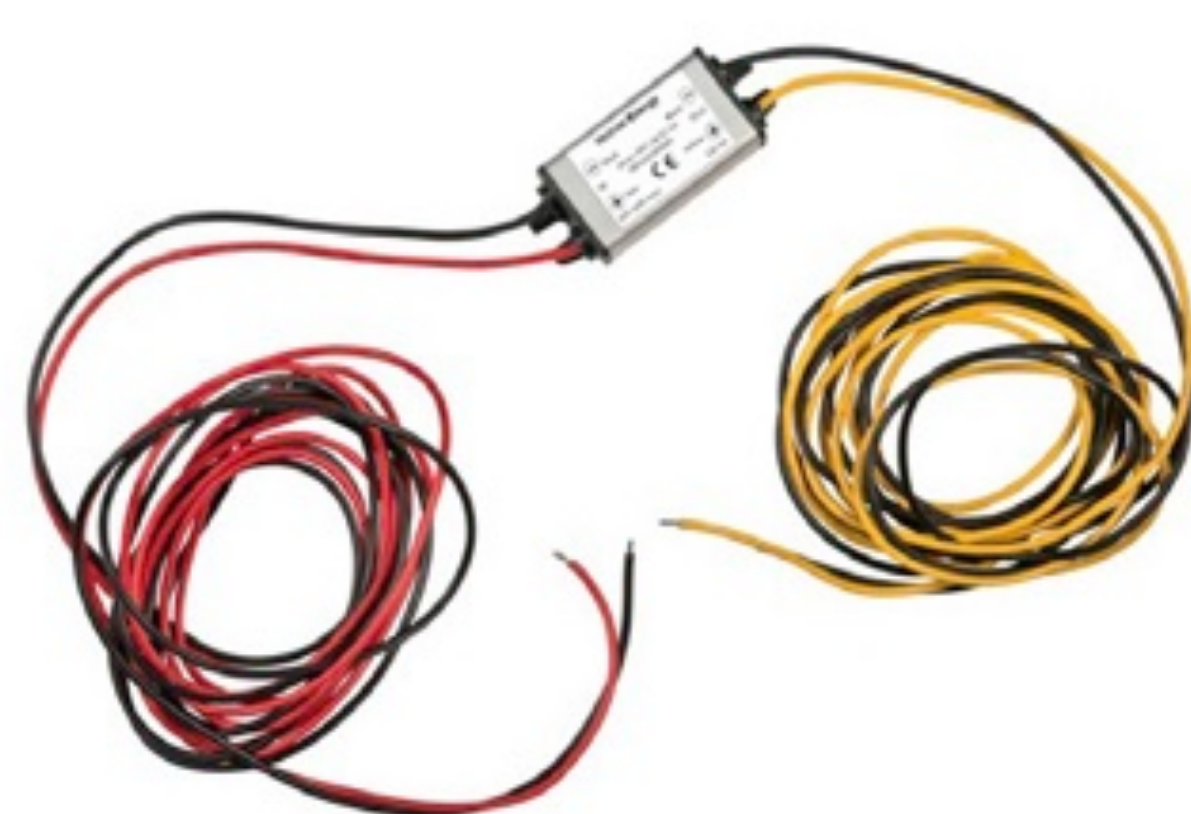
Orion IP67 24/12-5 with 1,8 m cables
