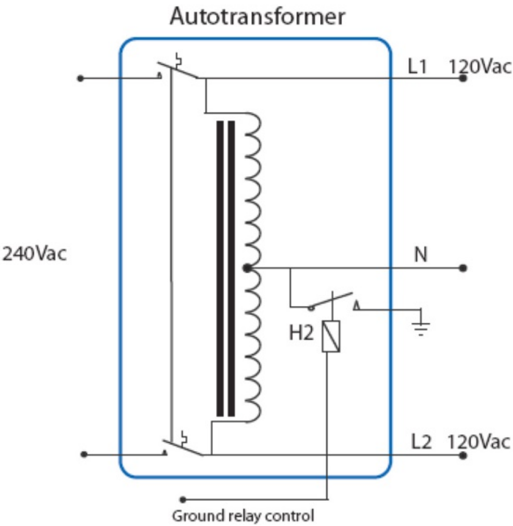
Autotransformer: schematic diagram
