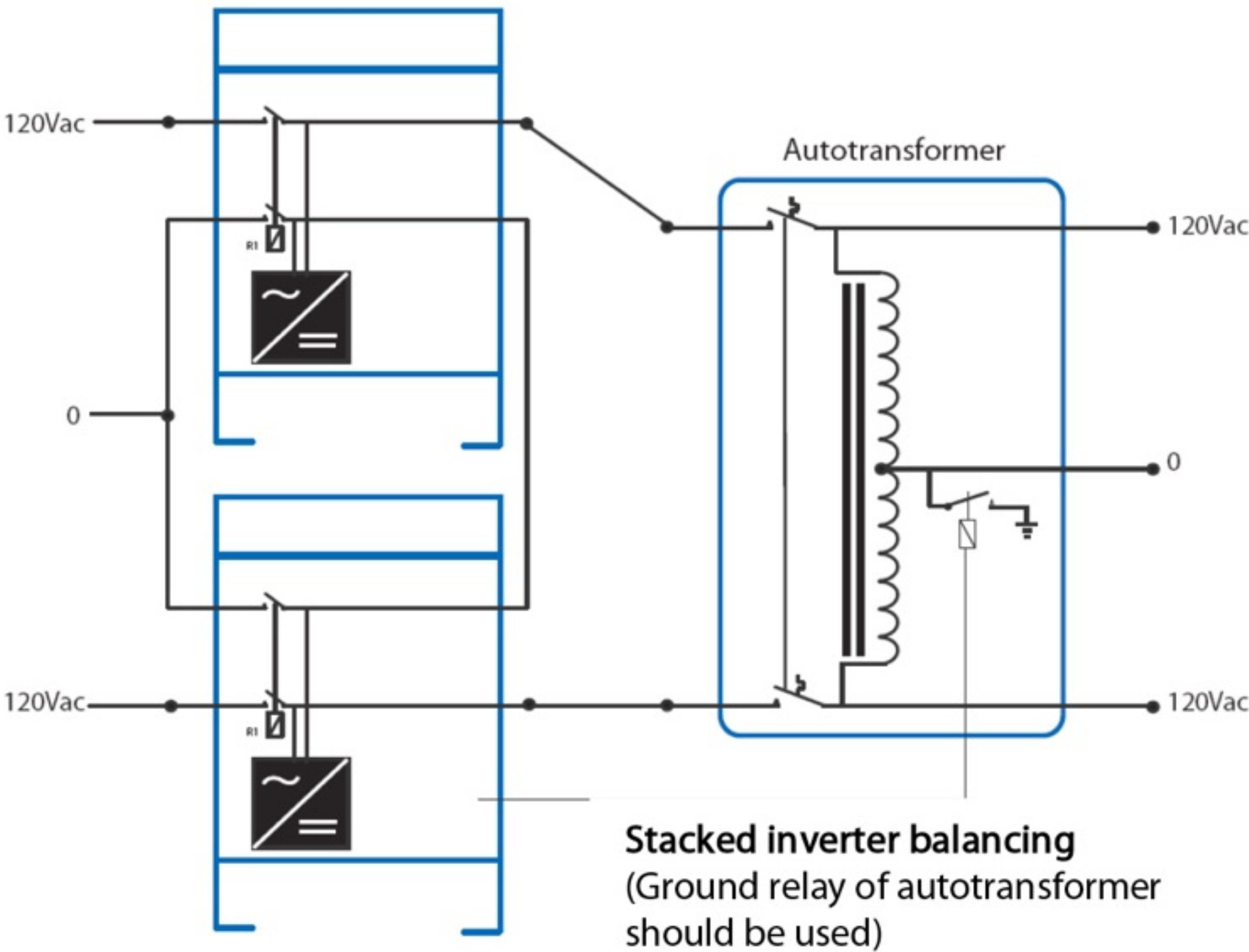
120/240Vac Generator
