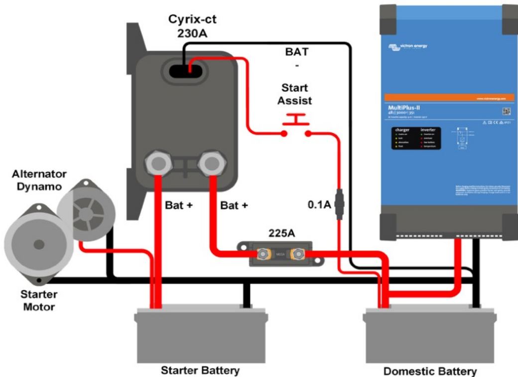
Cyrix-ct 12/24-230: connection diagram
