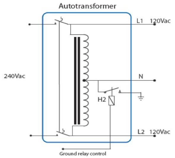
Autotransformer: schematic diagram
