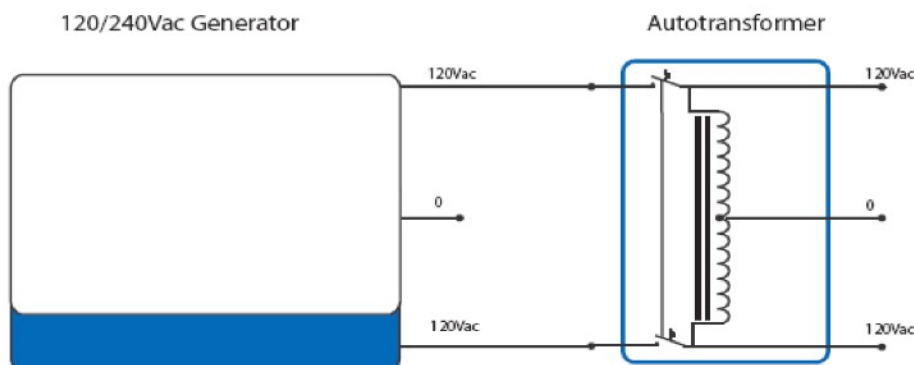
Stacked inverter balancing (Ground relay of autotransformer should be used)
